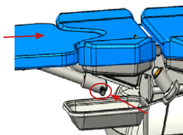
Fig. 3 Locking pin details
