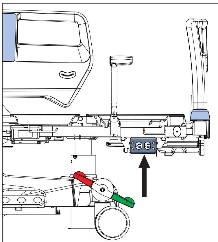
Fig. Position of the Auxiliary Outlet (120V)
