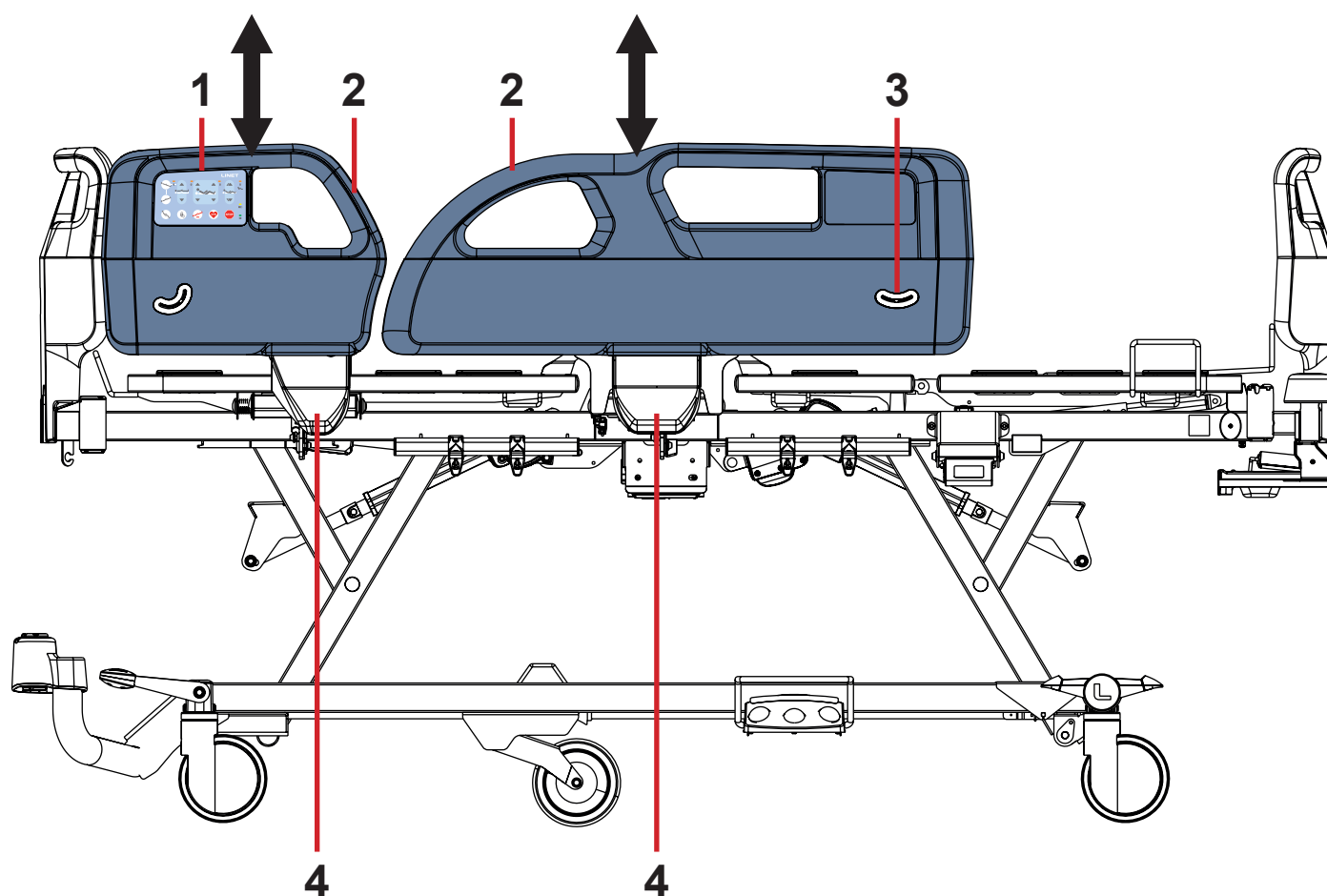
Fig. Plastic Siderail Description
