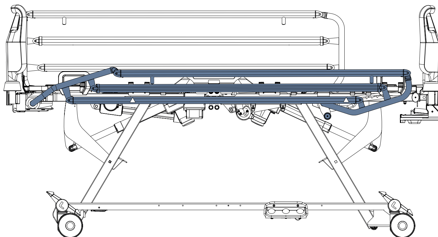
Fig. Right Single collapsible siderail in lower position
