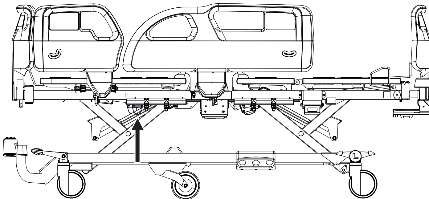
Fig. USB charger under the Backrest of the bed with plastic siderails
