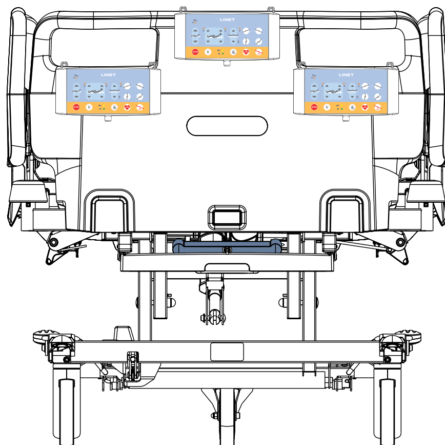
Fig. Correct positions of the Attendant Control Panel on the plastic foot board with one safety lock
