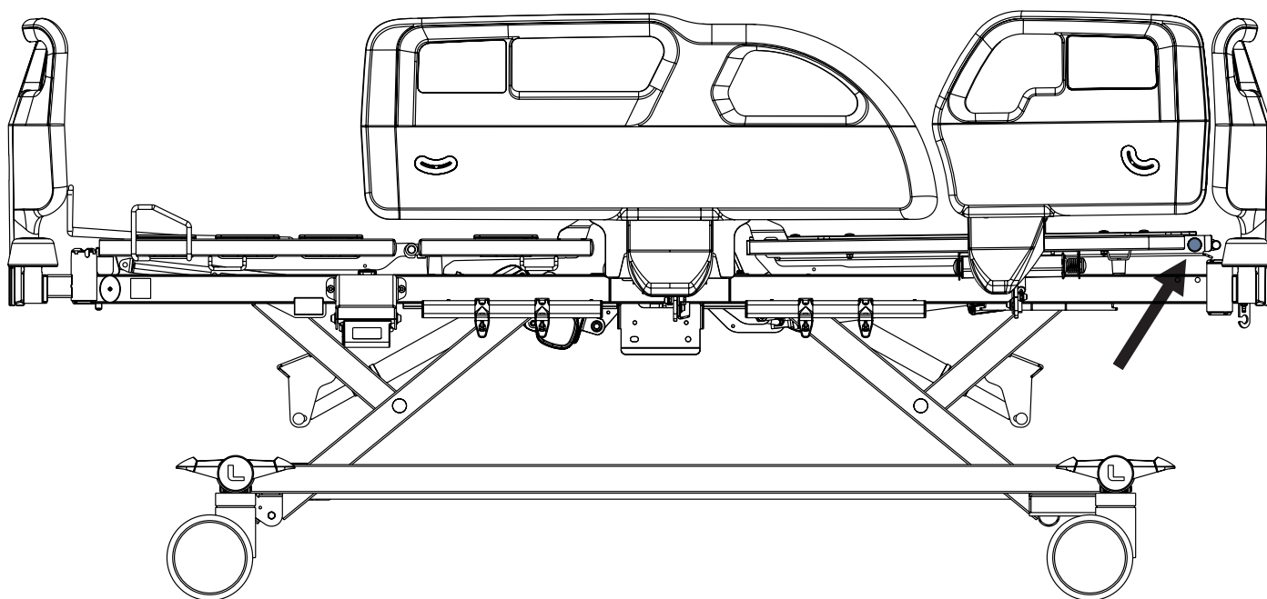
Fig. Position of the safety pin for fixing the X-ray cassette Holder
