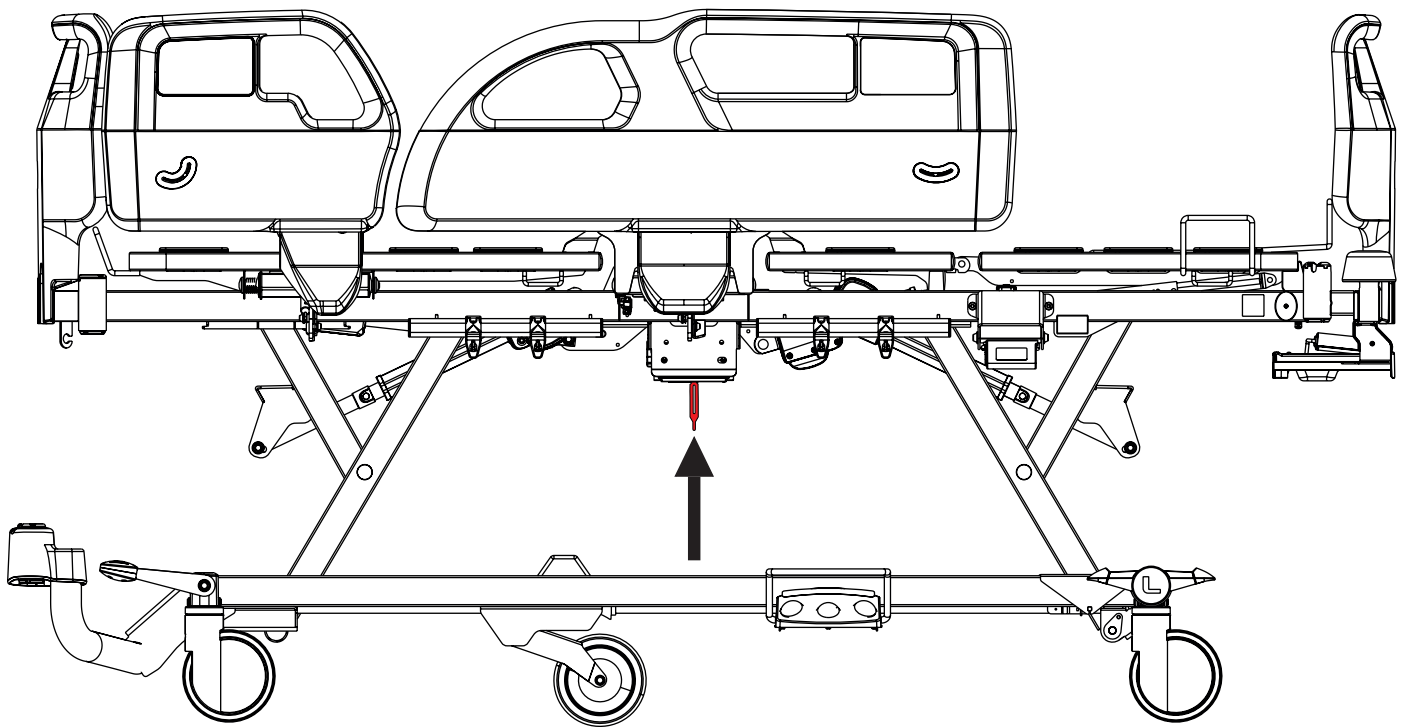
Fig. Position of Isolating Foil under the Backrest
