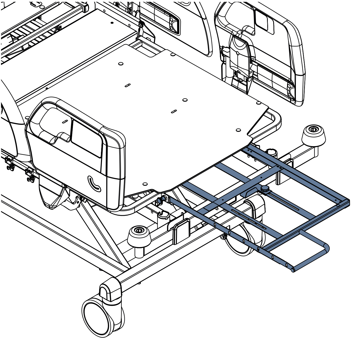
Fig. Pulled out X-ray cassette Holder in the most remote position
