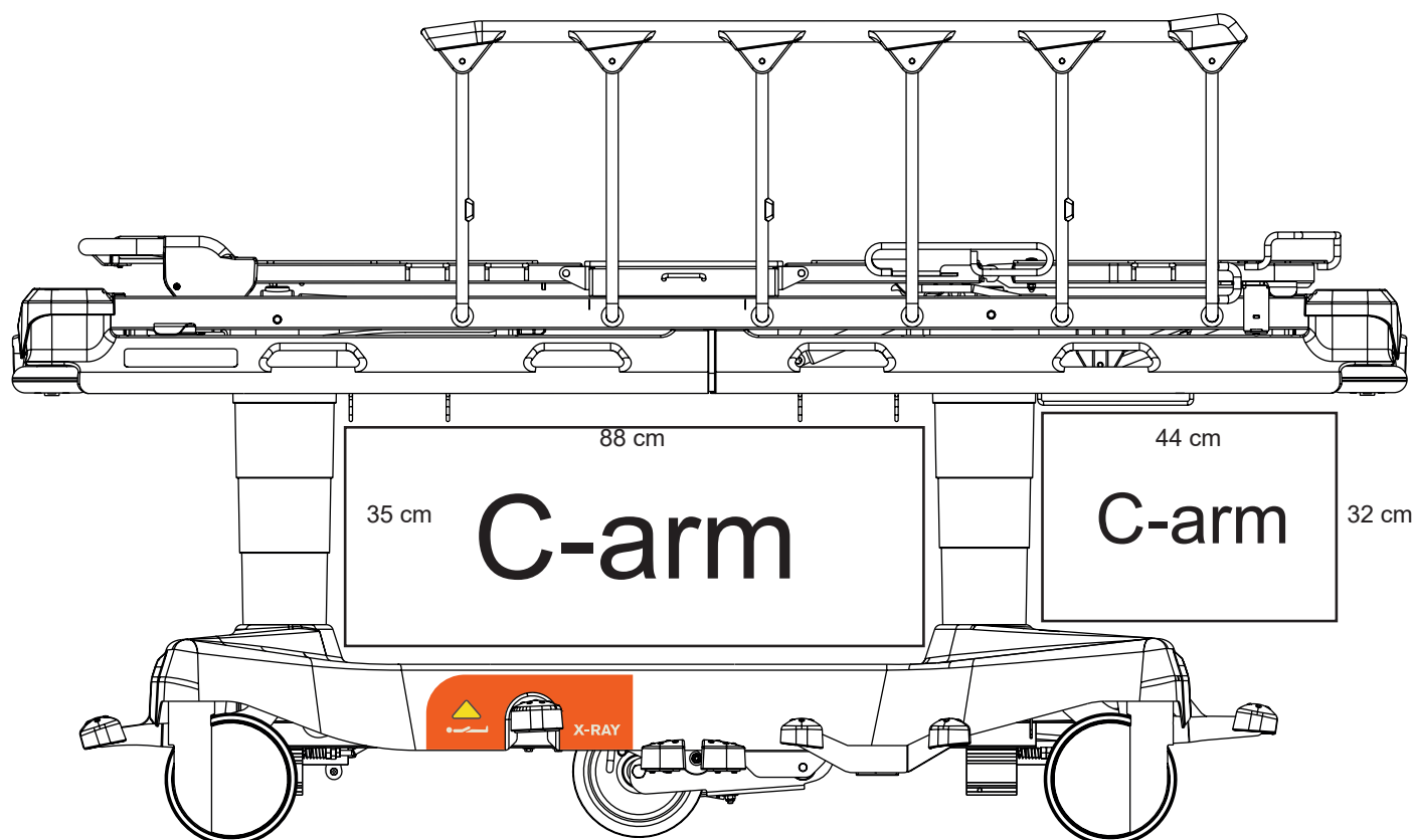
Fig. Space for the lower part of C-arm (Sprint 100 with Standard Mattress Support Platform)
