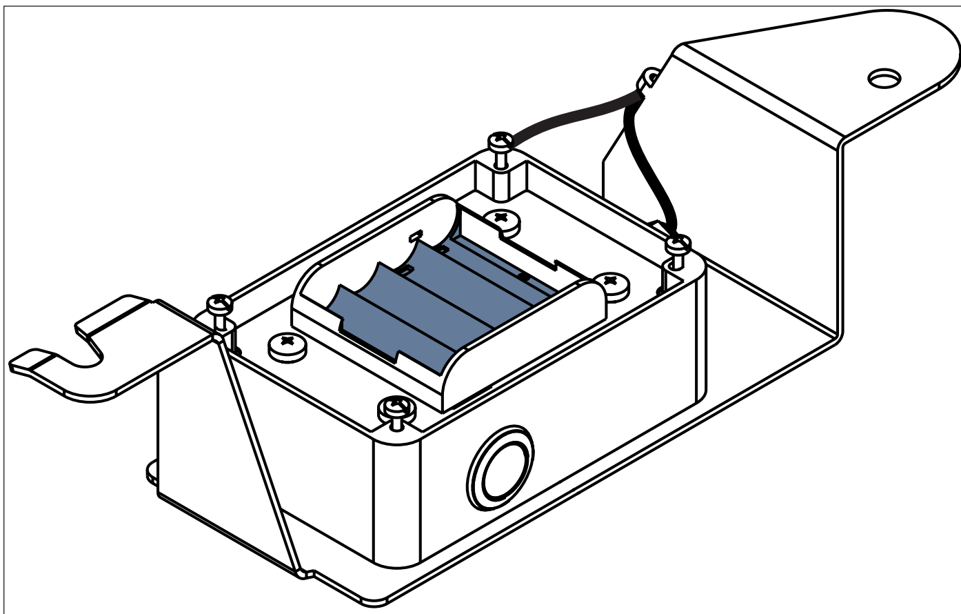
Fig. Opened Battery Box without batteries
