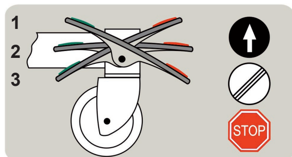
Fig. Central braking system lever
